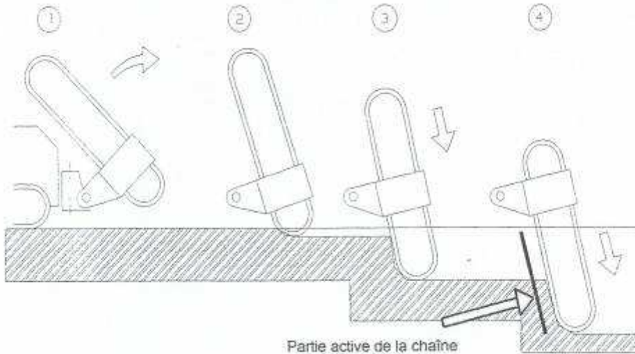
Working area of the cutting chain Parte active de la cadena
