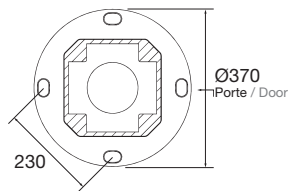
Semelle 4 tiges Base plate with 4 anchor bolts
