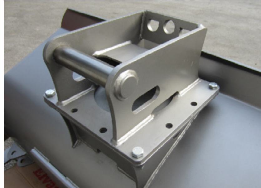
Changeable connection plate for all possible machines
