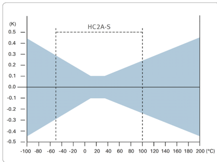
Temperature window graph for J115 probe
