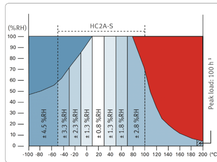
Humidity graph for J115 probe
