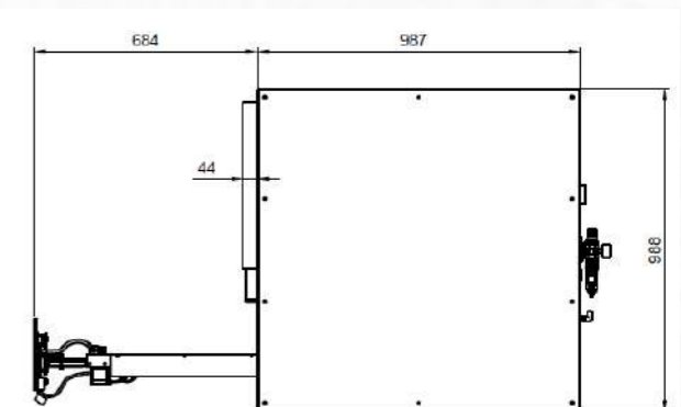
Top View Closed Cabinet
