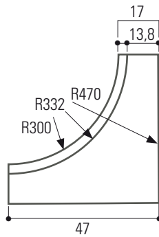
T3 concave
