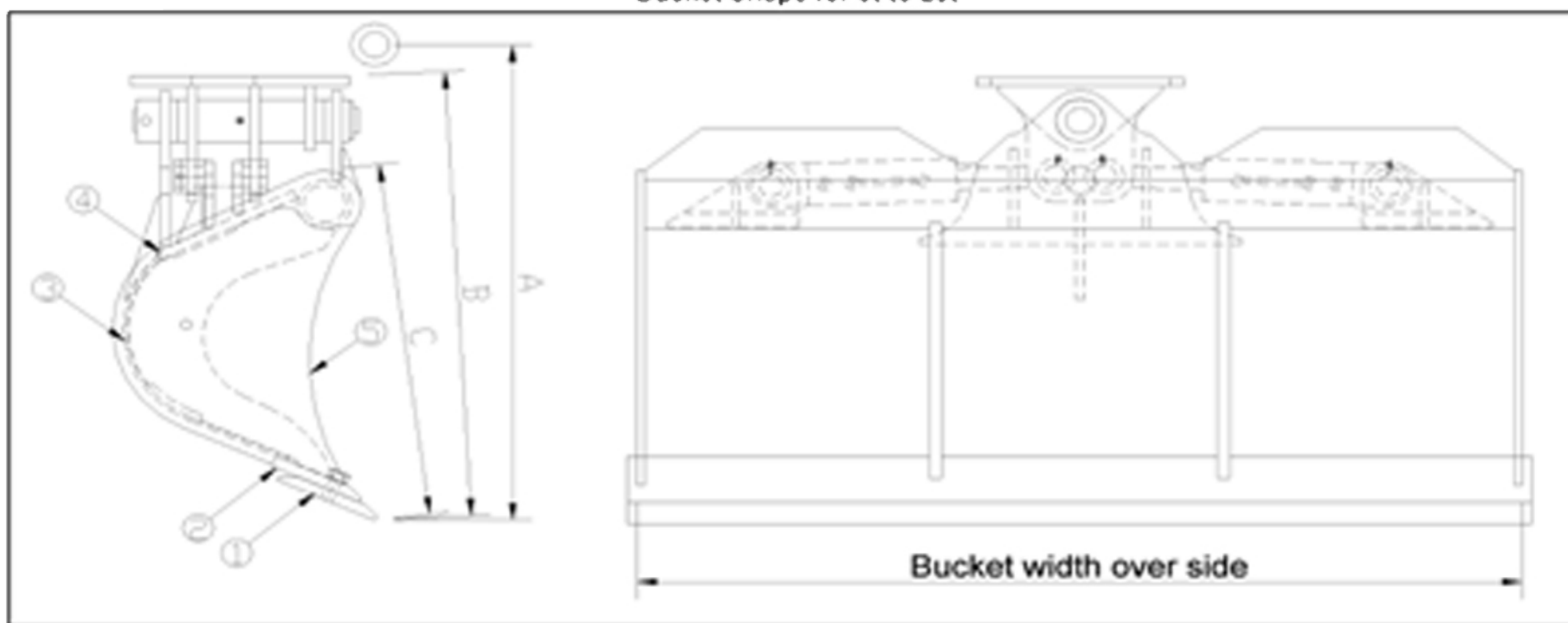
Bucket Shape for 8t to 25t
