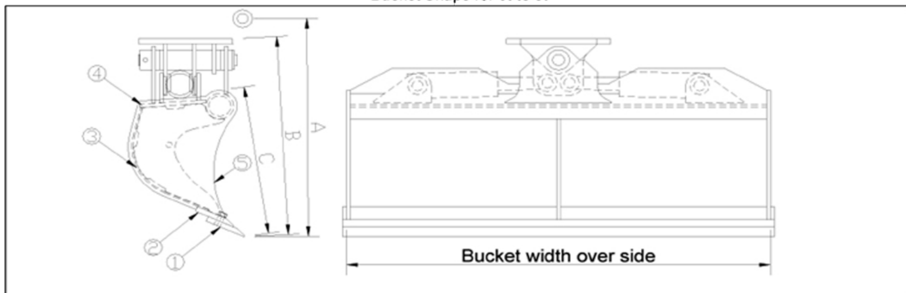
Bucket Shape for 8t to 25t
