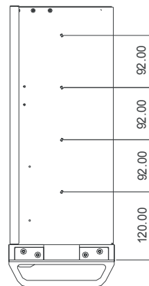
Right-side View
