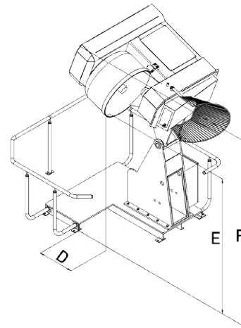
PE160FE-BASCUL234
