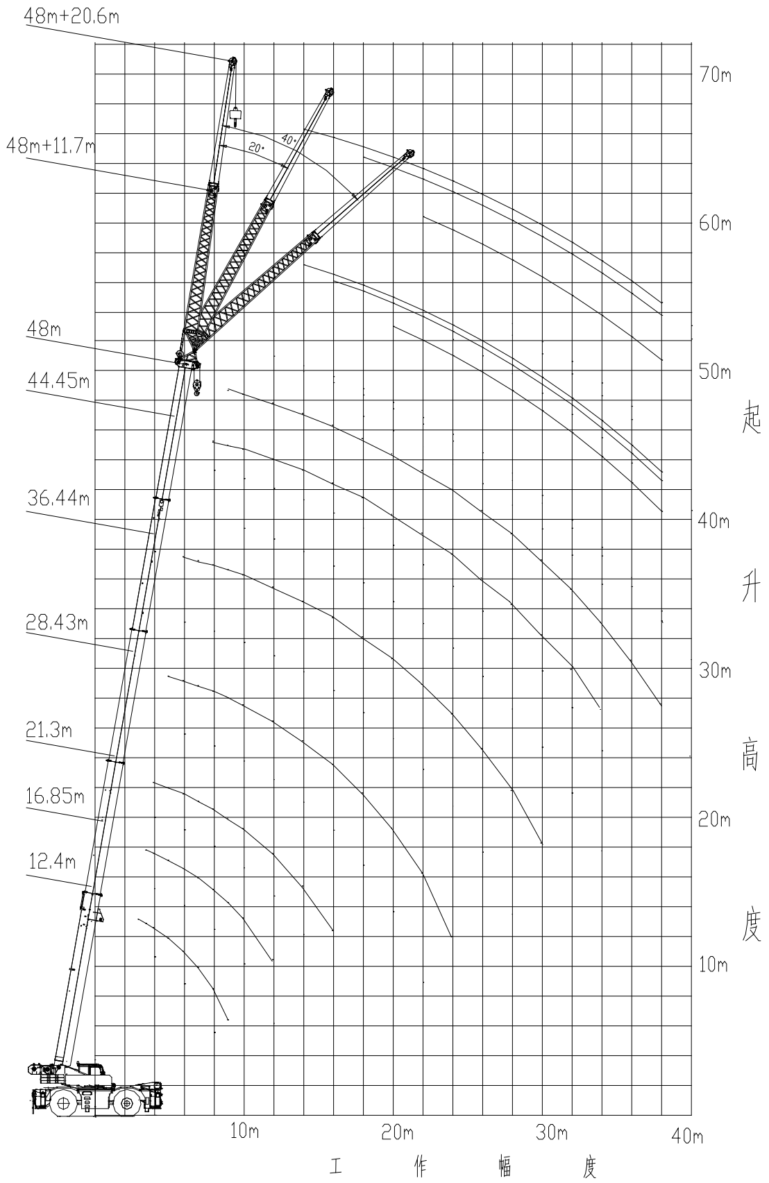
起升高度曲线 Lifting height curves
