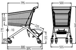
02 DIMENSIONS DES CHARIOTS LIBRE-SERVICE
