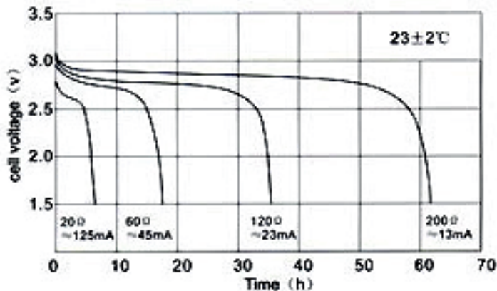
Load-Capacity Characteristics
