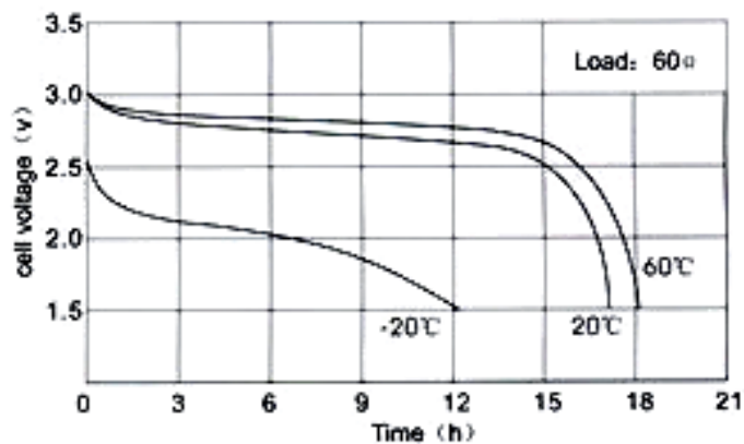
Temperature Characteristics
