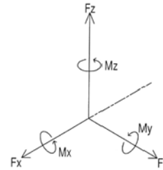
Figure 11 Forces et moments maximum applicables aux brides
