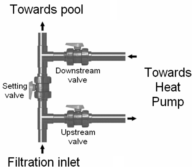
By-pass diagram
