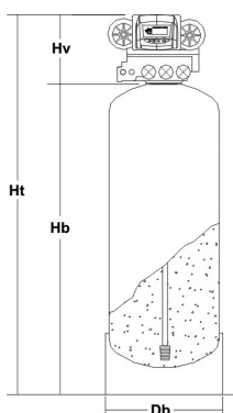
Vanne Autotrol Magnum
