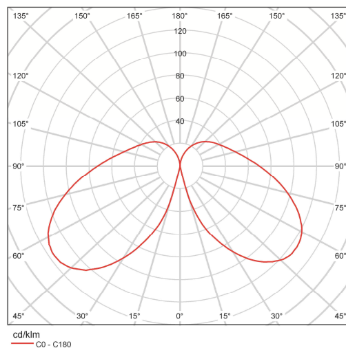
Courbe de distribution KARIN 900 LED
