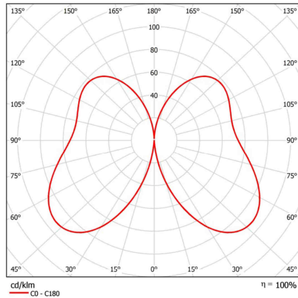
Distribution curve KARIN 4800 LED
