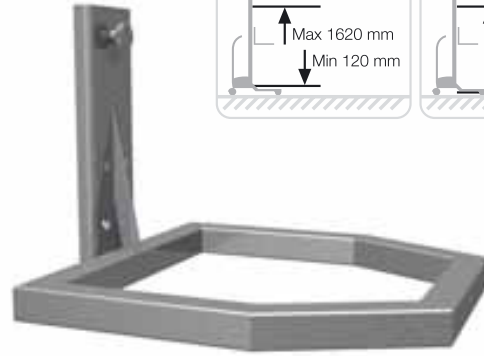
2. Frame 8832 for platform 8831C (410x400 mm). Including quick-coupling system.
