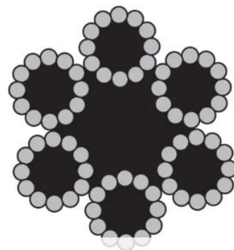
Steel wire rope 6x12+7FC
