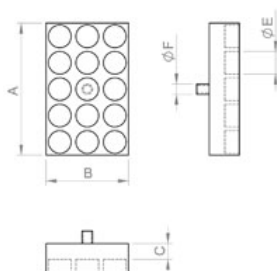
Version 96 trous
