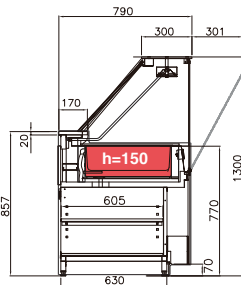
VELSBM -VDA banho-maria bain-marie bain-marie baño maria
