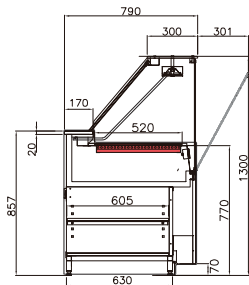
VELSTA -VDA tampo aquecido heated deck plateau chaud tampo caliente
