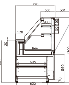
VELSNT - VDA neutra dry ambient neutre neutra
