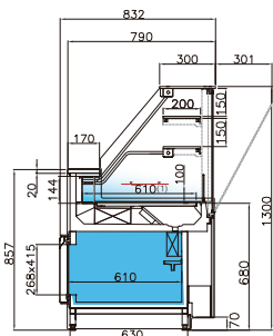
VELSVT - VDA 3M2 (1) ventilada total total ventilated ventilée total ventilada total
