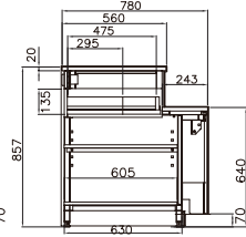
ELCX2N caixa support counter caisse caja
