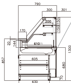
VELSNTV - VDA neutra "ventilada" "ventilated" dry ambient "ventilée" neutre "neutra" ventilada
