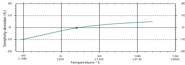
Fig 13 : Sensitivity deviation versus temperature
