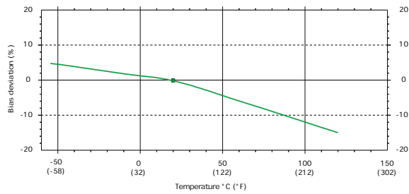
Fig 12 : DC (Bias) deviation versus temperature
