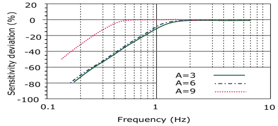
Fig 14b : Low Frequency response, amplitude
