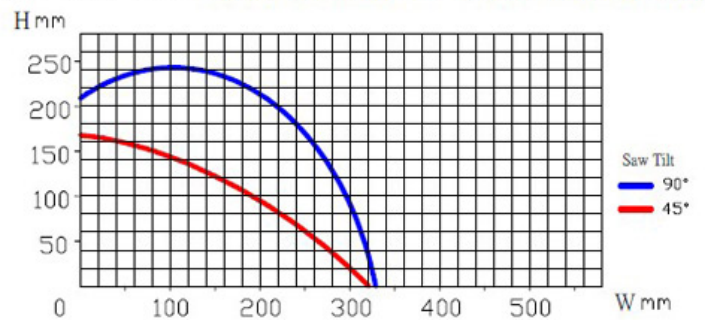
T5/T5S 26" Work Table rotary 45° Cutting Capacity Chart
