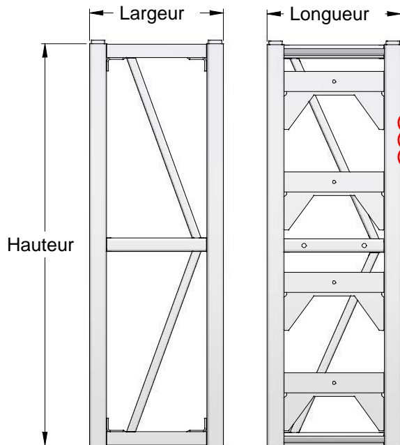
Figure C.1 Section de mât
