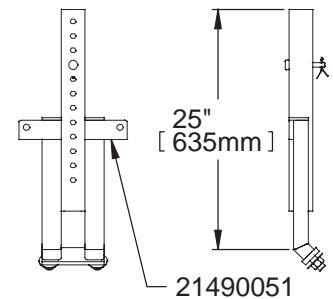
Figure C.19 Attache murale en angle
