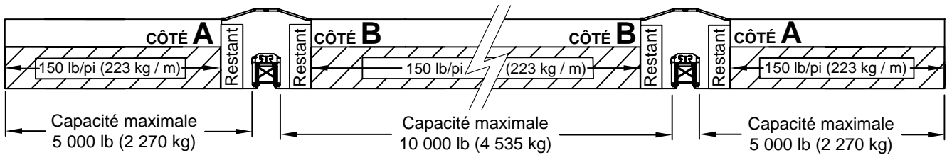
Figure A.3d Configurations (maçonnerie)
