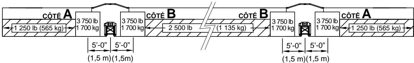
Figure D.1e Configurations (autres)
