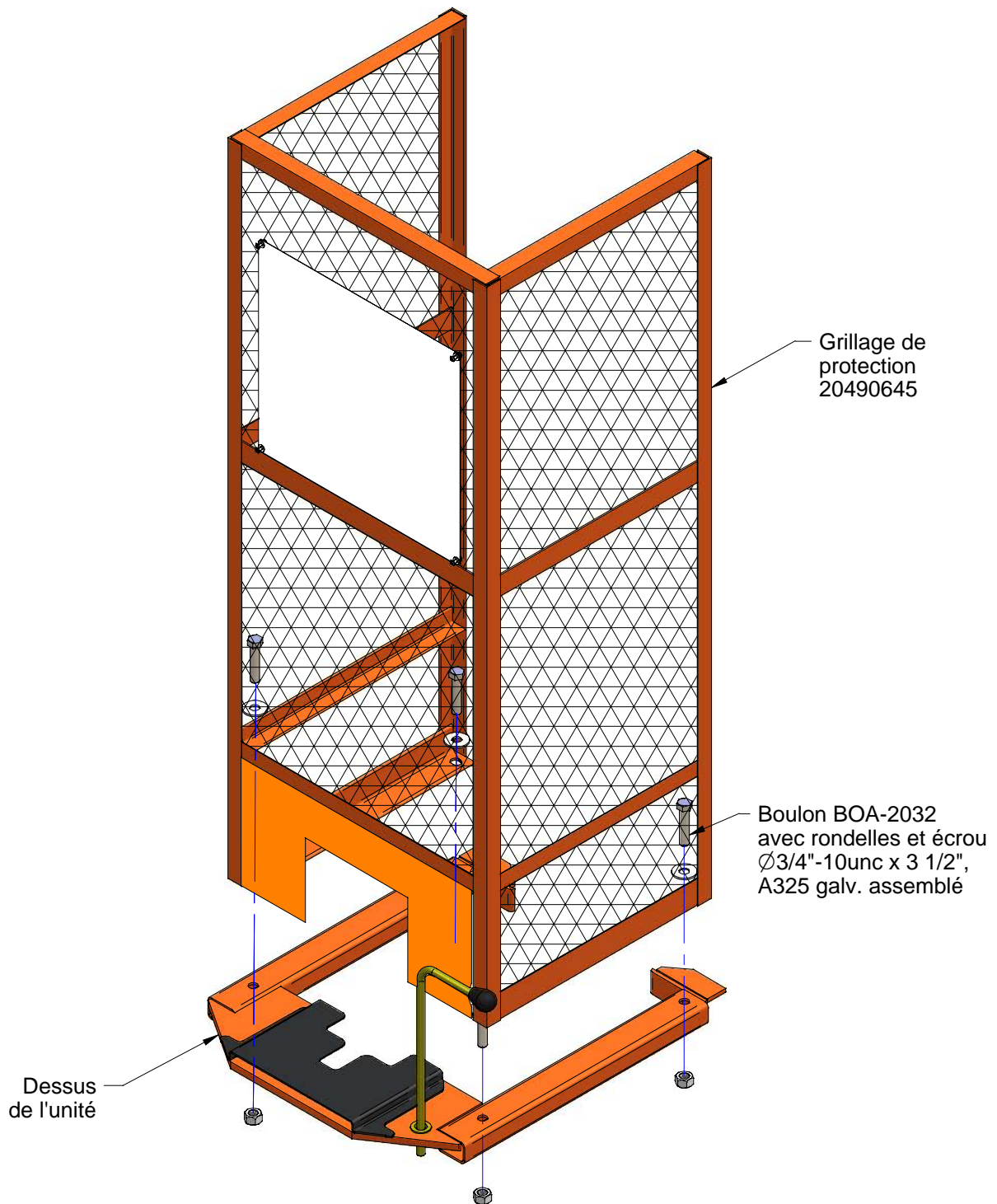
Figure B.5 Grillage de protection
