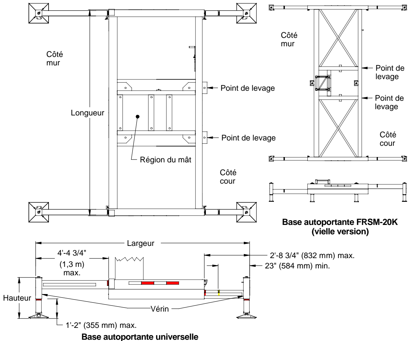
Figure B.3 Dimensions de la base autoportante
