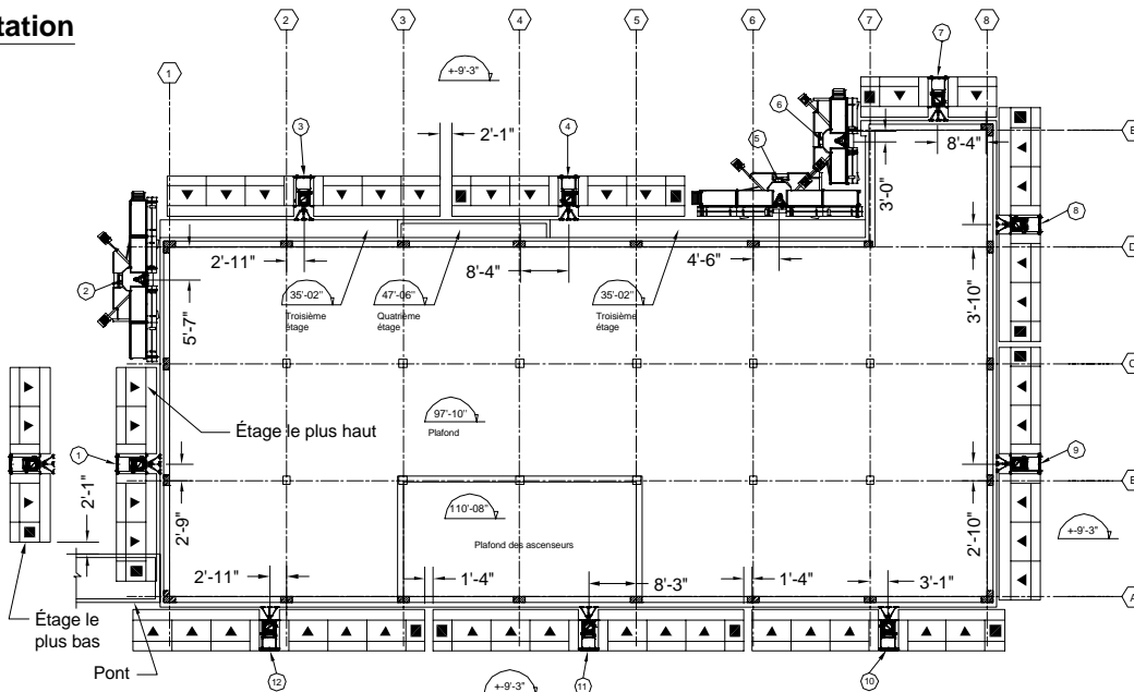
Figure B.6 Implantation
