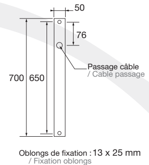
MURALE / CONTRE POTEAU / WALL-MOUNTED / AGAINST A POST
